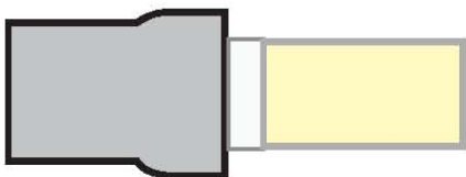
100 mm DWV Pipe Socket to 90mm S/W Pipe Spigot
